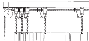
Back-Pack Guides and trim chains installed
