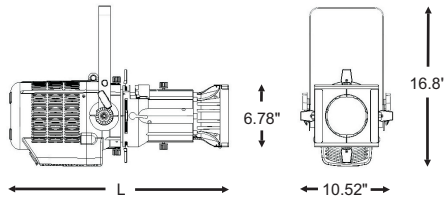
PHX1 LED Spot, Fixed Focus 35° "L" Length varies with lens size
