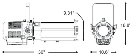
PHX LED Spot, Zoom Focus 15°-35°
