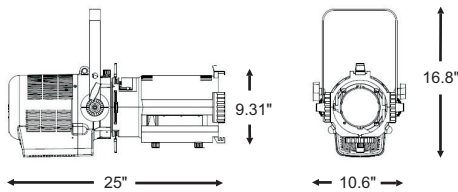
PHX LED Spot, Zoom Focus 30°-55°
